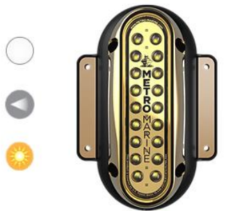
F-SME1-V-W3-45 Surface Mount
